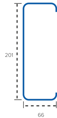
DIAGONAL TIES
